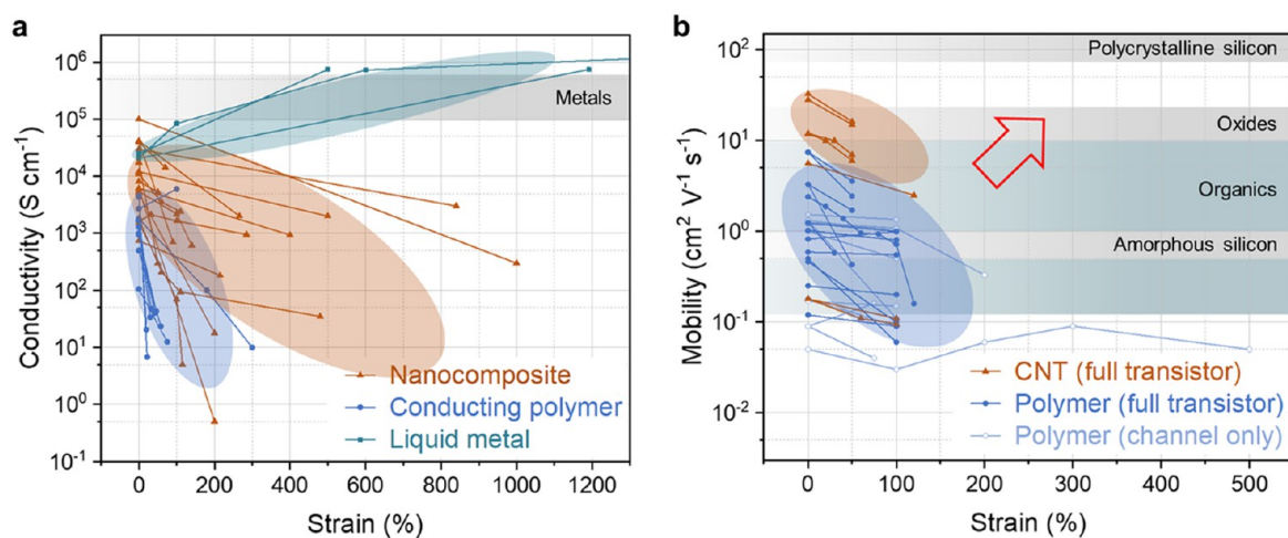
Figure 7. Performance of intrinsically stretchable (a) conductors and (b) semiconductors. (a) Intrinsically stretchable conductors are realized in three materials categories: nanocomposites, conducting polymers, and liquid metals; ionic conductors are not included. Conductivities of stretched liquid metals are calculated from resistance changes under unidirectional strain, based on the assumption of incompressible solid undergoing uniform deformation. Non-stretchable bulk metals are plotted in the gray band for comparison. Values extracted from refs 269, 285, 329–345. (b) Stretchable semiconductors are based on semiconducting CNTs or conjugated polymers. Mobility measurement was done in either stretched materials transferred to non-stretchable substrates (channel only) or fully stretchable transistors and transistor arrays (full transistor). Values for stretch directions both parallel and perpendicular to the channel length are included. Typical mobilities of common non-stretchable semiconductors are plotted in bands for comparison. 346 Red arrow indicates area for improvement. Values extracted from refs 323, 324, 347–364.
