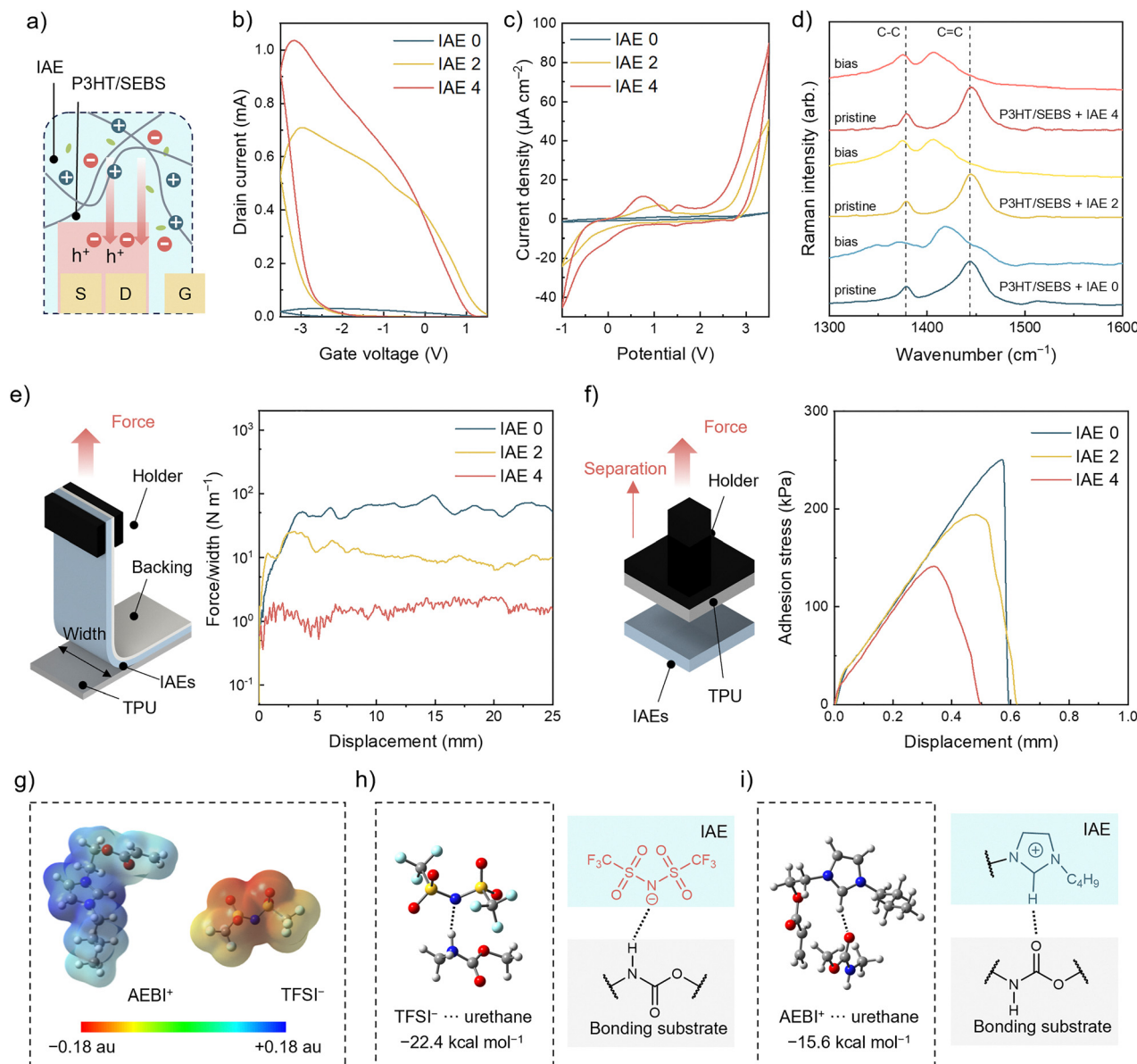
Fig. 2 Design of IAEs for electrolyte-gating of IONTs. (a) Schematic illustration of the electrolyte-gated operation mechanism of the IONT. (b) Transfer curves of IONTs using IAE0, IAE2, and IAE4 as electrolytes. (c) Cyclic voltammetry performed using three IAEs as electrolytes (arrows indicate the oxidation peaks). (d) In situ Raman spectra of the P3HT/SEBS channel before and after applying gate bias using three IAEs as electrolytes. (e) 90°-peel test results (force per width vs. displacement) of three IAEs on TPU substrates. Schematic: test setup. (f) Tack test results (adhesion stress vs. displacement) of three IAEs on a TPU substrate. Schematic: test setup. (g) Electrostatic potential surfaces of AEBI + and TFSI - , calculated using DFT. Color scale: positive (blue) to negative (red) potential. DFT calculations of binding energies between (h) TFSI - -urethane and (i) AEBI + -urethane with schematic representations of interfacial interactions.
