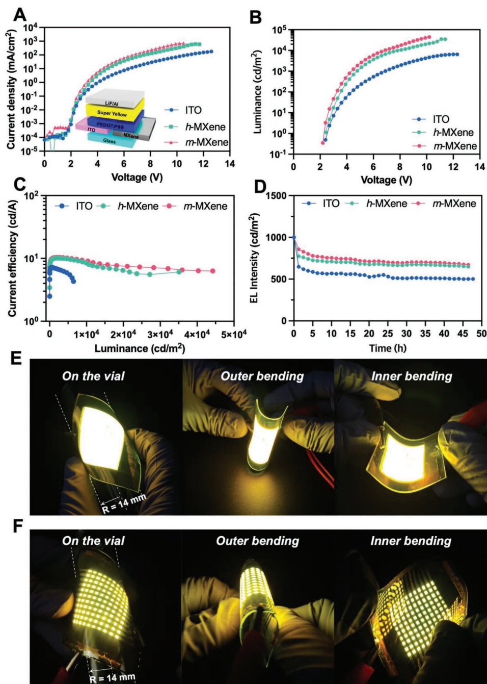
Figure 4. A) Current density vs voltage ( J - V ), B) luminance vs voltage ( L - V ), C) current efficiency, and D) lifetime (operated at 1000 cd m -2 initial luminance) curves for ITO, h -MXene, and m -MXene-based OLEDs. E,F) Digital photos of h -MXene-based large-area solid-state lighting (E) and 10 × 10 passive matrix (F) on PET flexible substrates (6 cm × 6 cm) operated under different mechanical deformations.
